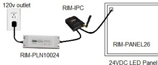
Connection Diagram
